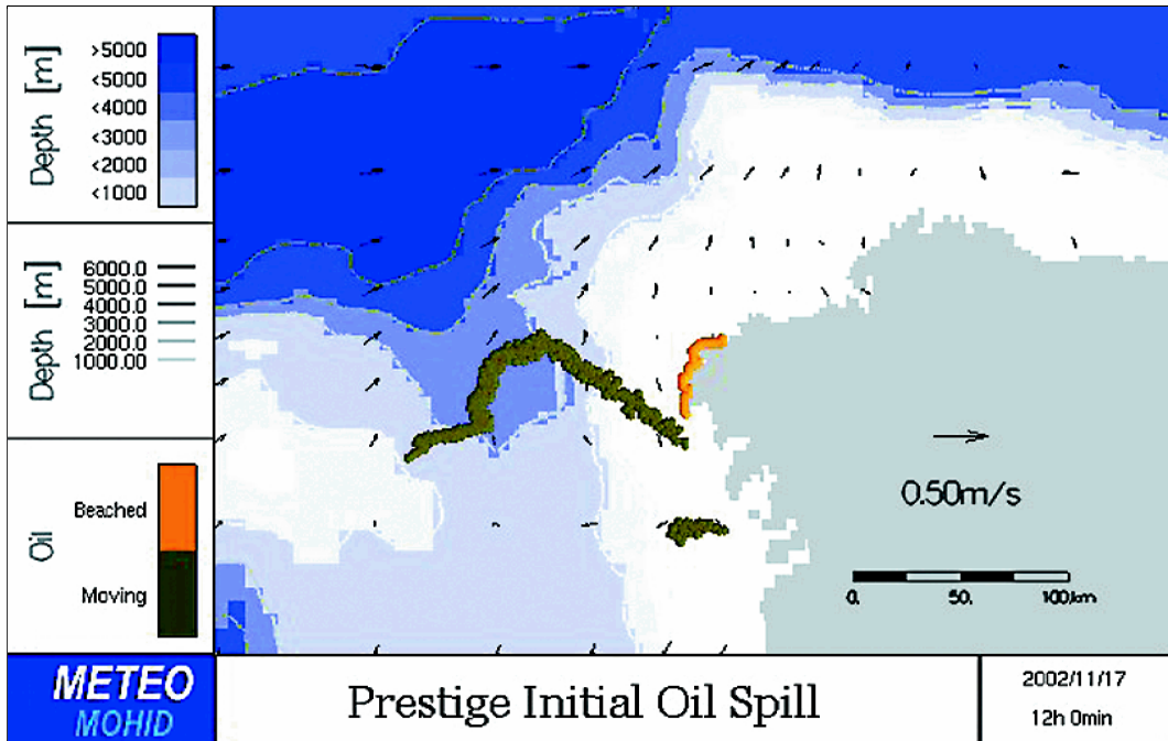
Fig. 7 METEO–MOHID results with continuous emission for 1200 GMT on 17 November 2002 (see article on p. 452).
