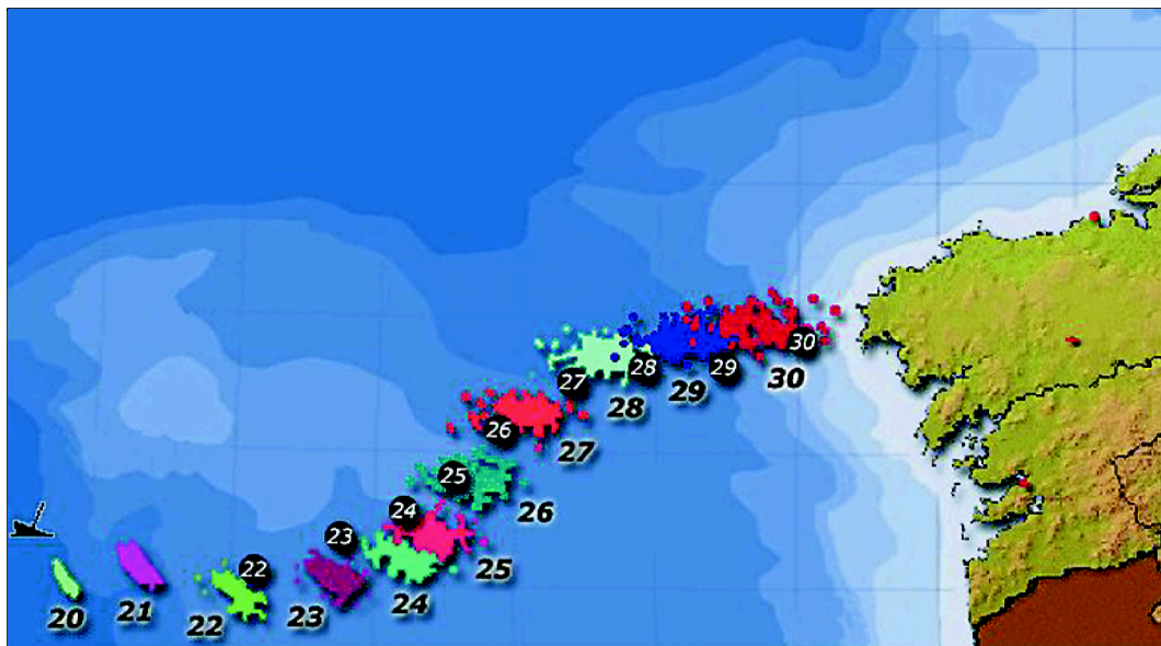
Fig. 8 Comparison between METEO–MOHID daily results (coloured spots with the respective forecast day as a black number) and the observed daily maximum fuel concentration (number inside black circle). Symbol lower left indicates the place of the Prestige sinking. (See article on p. 452.)
